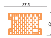
Porotherm 25/37.5 AKU
